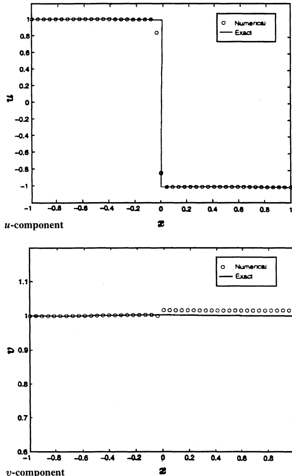
Fig. 2 For a second-order ENO scheme, u and v components of Eq. (9).
